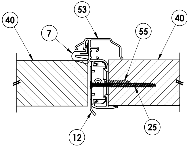
1 5 HORIZONTAL CROSS SECTION Outswing Shown (Inswing Similar)
