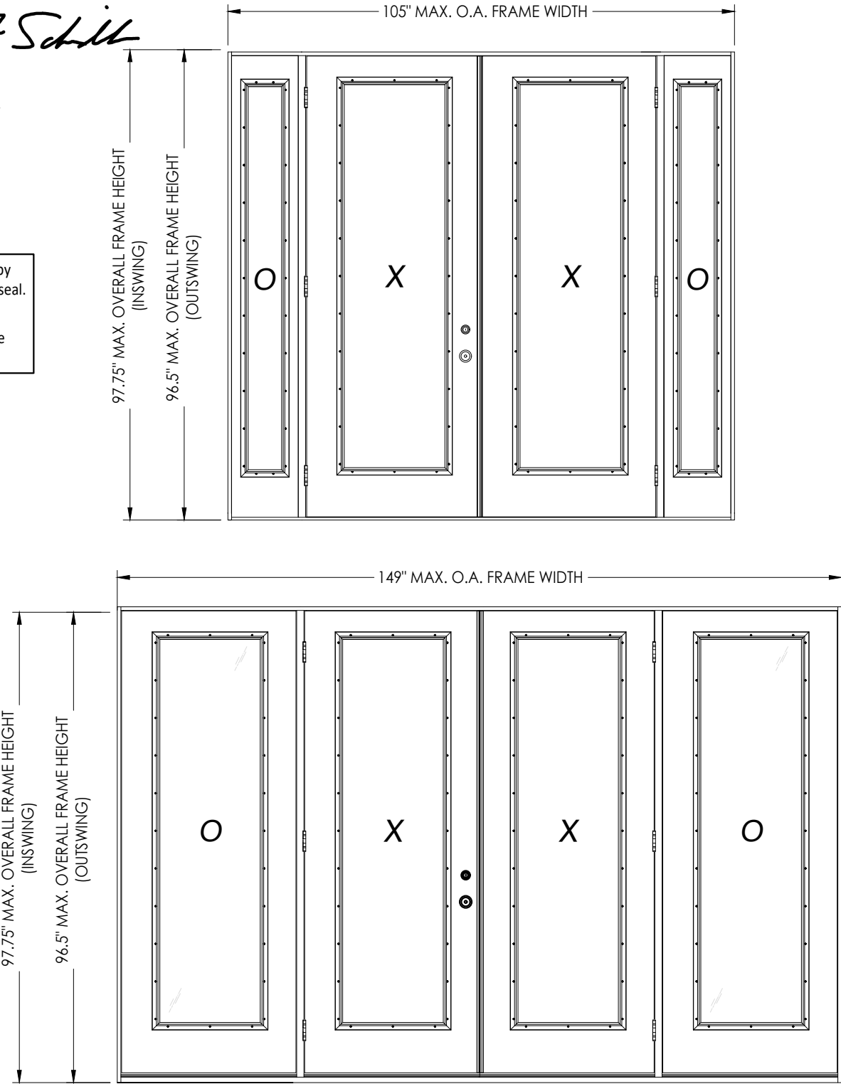
OXO CONTINUOUS HEAD & SILL
