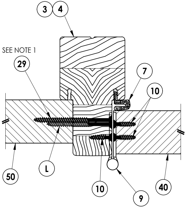
2 5 HORIZONTAL CROSS SECTION Outswing Shown (Inswing Similar)
